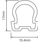
PR17D • P17 Recessed Profile
