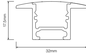
PR17D • P17 Recessed Profile
