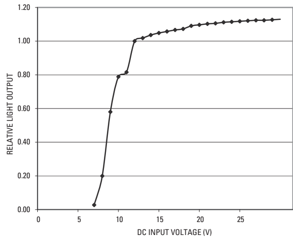
G4 LED CG4-095B-V2 RELATIVE LIGHT OUTPUT
