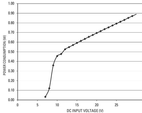
G4 LED CG4-095B-V2 POWER CONSUMPTION
